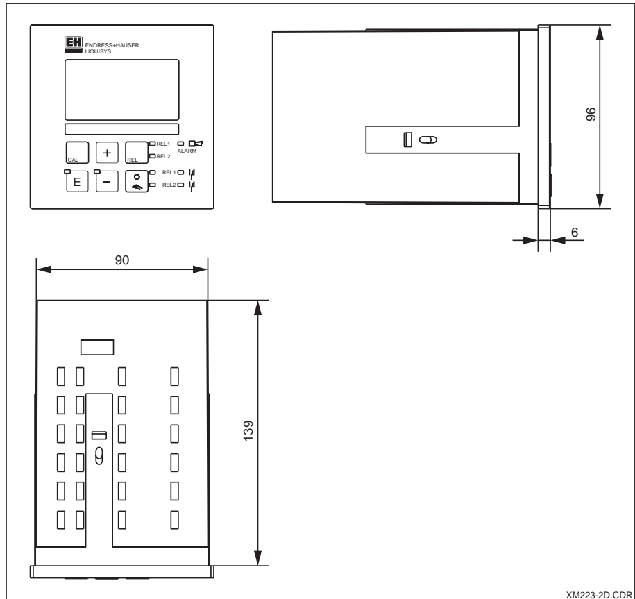
Dimensions of Lquisys M CUM 223
