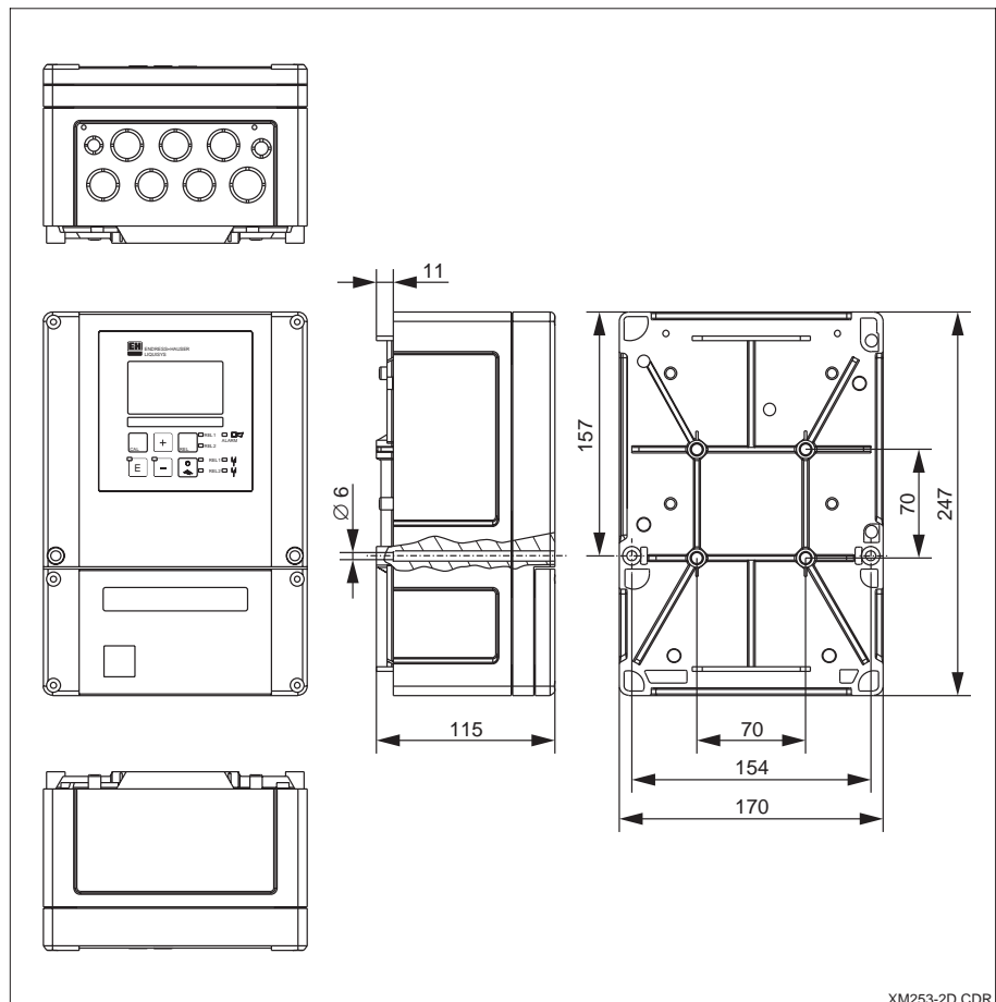
Dimensions of Lquisys M CUM 253
